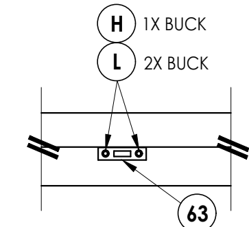
DETAIL 1 Surface Bolt Strike @ Head Outswing
